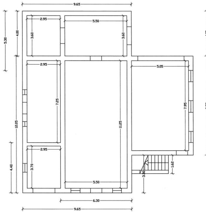
Piano terra
