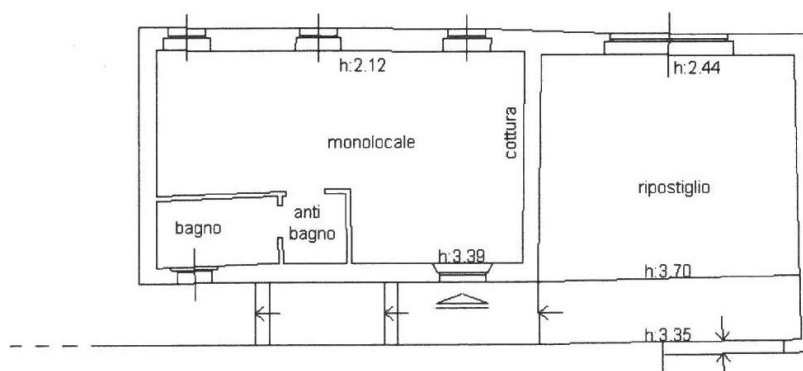
PIANO TERRA
