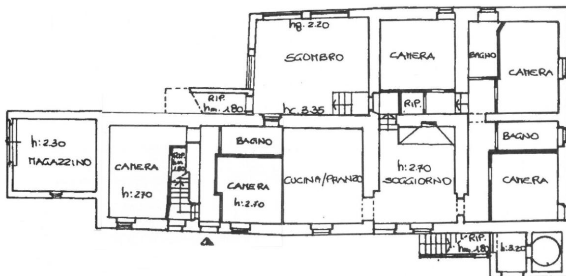
PIANO TERRA
