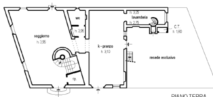
PIANO TERRA
