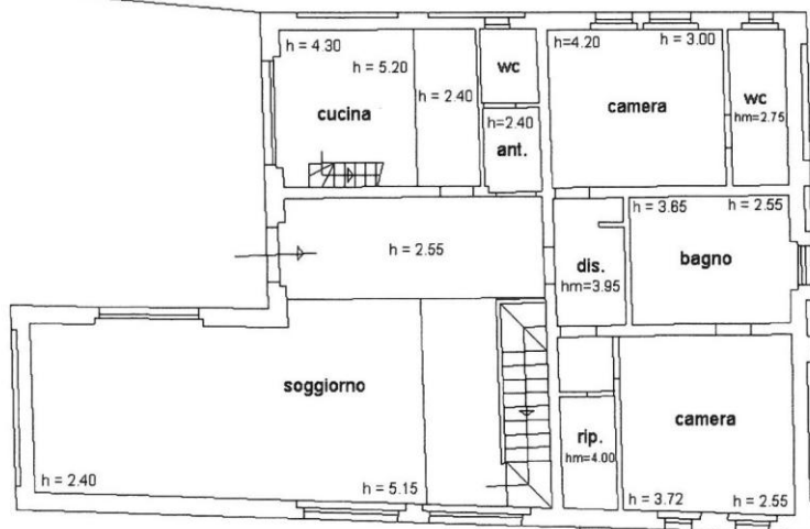
PIANO TERRENO
