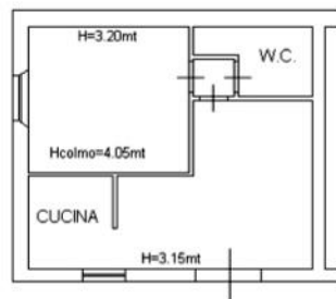
PIANO TERRA
